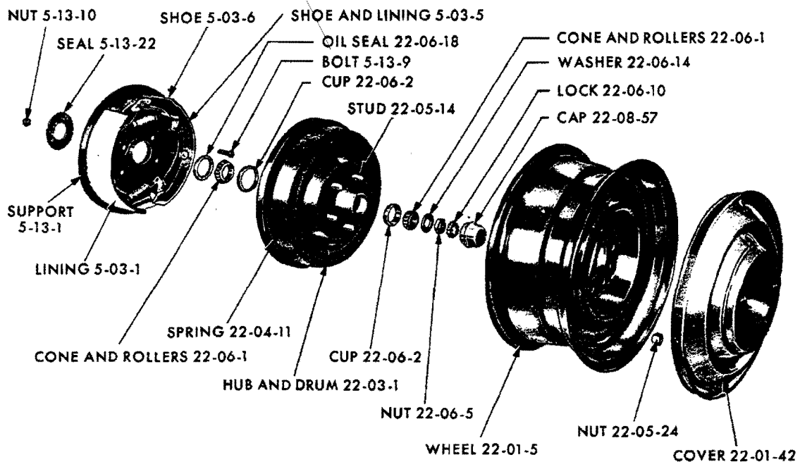
FRONT WHEEL
