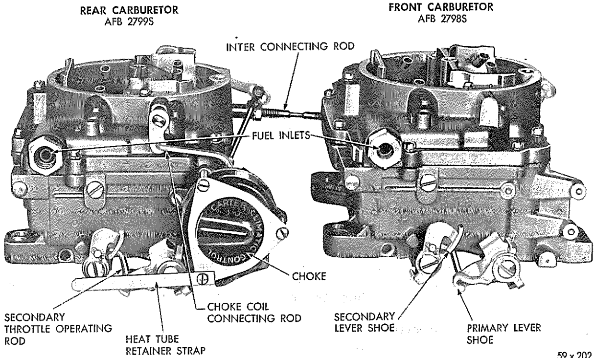
Fig. 8 - Front and Rear Carburetors (Right Side View)
