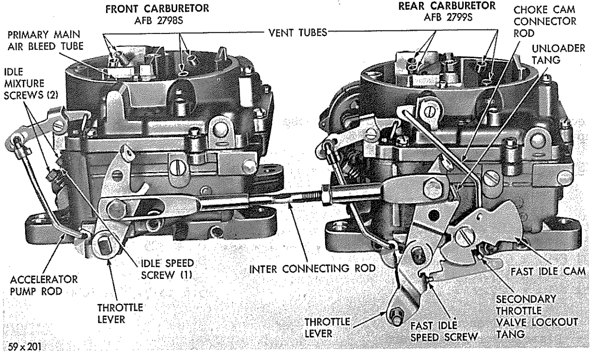
Fig. 7 - Front and Rear Carburetors (Left Side View)
